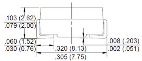
Package Outline Dimensions in Inches (Millimeters) 封装外观尺寸单位英寸 (毫米)
