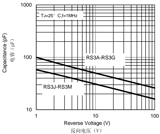
Fig. 3 - Typical Junction Capacitance 图3 典型的结电容
