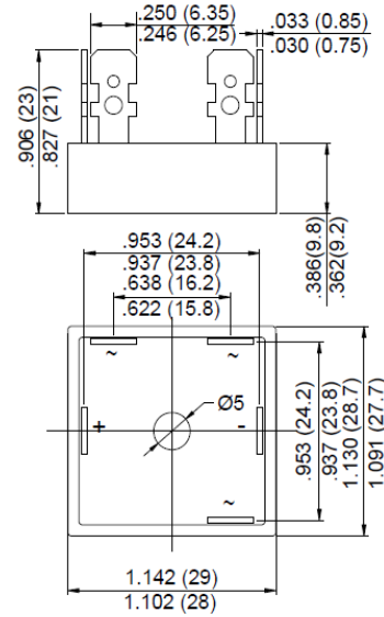
Package Outline Dimensions in Inches (Millimeters) 封装外观尺寸单位英寸 (毫米)
